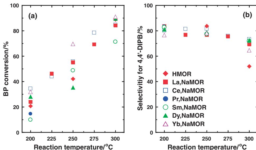
Figure 6. Effects of temperature on the isopropylation of BP over Ln,NaMORs. (a) The activities, (b) the selectivities of 4,4'-DIPB. Reaction conditions: BP, 100 mmol; catalyst, 0.5 g; propene, 0.8 MPa; temperature, 200–300 °C; period, 4 h.
