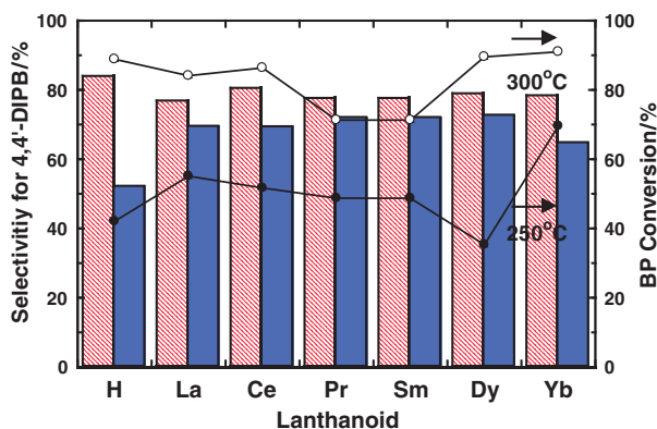
Figure 7. Effects of temperature on the isopropylation of BP over Ln,NaMORs. Reaction conditions: BP, 100 mmol; catalyst, 0.5 g; temperature, 250 and 300 °C; propene pressure, 0.8 MPa; period, 4 h. Legend: \square : 250 °C; \blacksquare : 300 °C.
