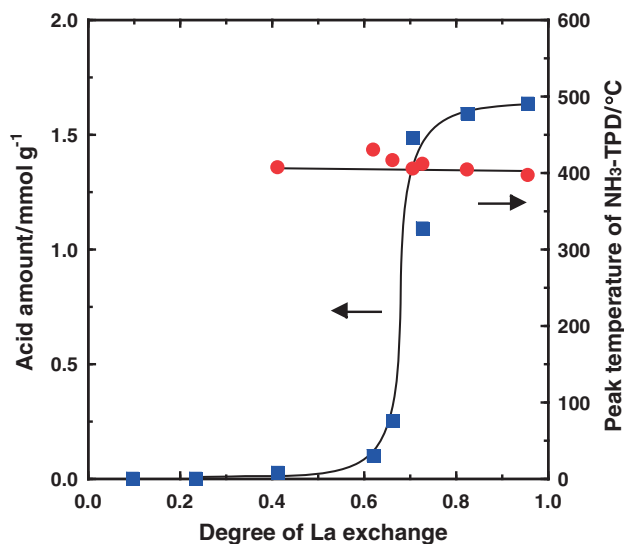
Figure 2. Effects of acid amounts and peak temperature of \text{NH}_3 -TPD on \text{La,NaMOR} .
