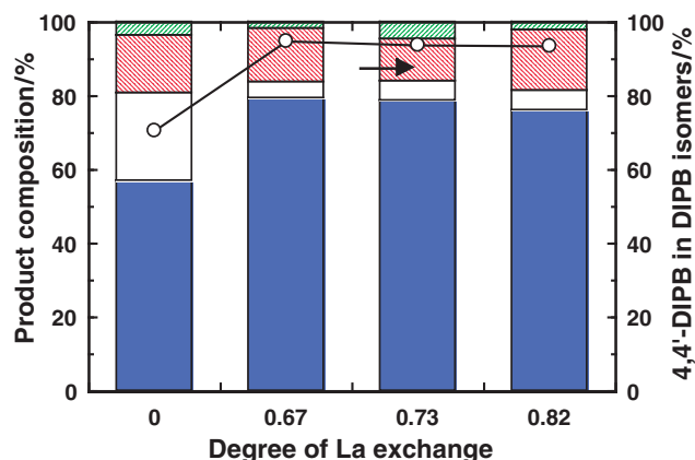
Figure 5. Effects of the isomerization of 4,4'-DIPB on degree of cation exchange of La,NaMOR. Reaction conditions: 4,4'-DIPB, 50 mmol; catalyst, 0.5 g; propene, 0.8 MPa; temperature, 300 °C; period, 4 h. Legend: ■: 4,4'-DIPB; □: 3,4'-DIPB; ■: TriIPB; ■: IPBP.
