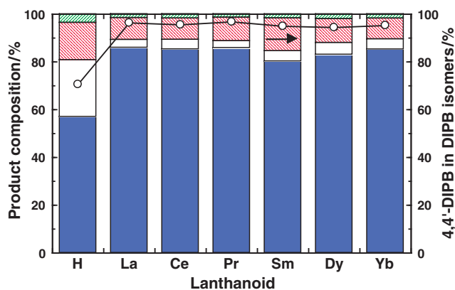
Figure 8. The isomerization of 4,4'-DIPB over Ln,NaMORs. Reaction conditions: 4,4'-DIPB, 50 mmol; catalyst, 0.5 g; temperature, 300 °C; propene pressure, 0.8 MPa; period, 4 h. Legend: the same as in Figure 5.
