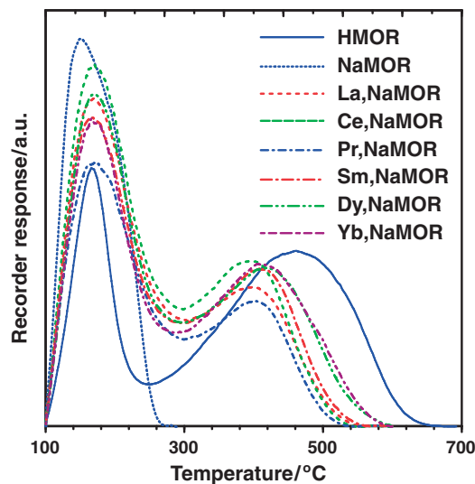
Figure 3. \text{NH}_3 -TPD profiles of \text{Ln,NaMORs} .
