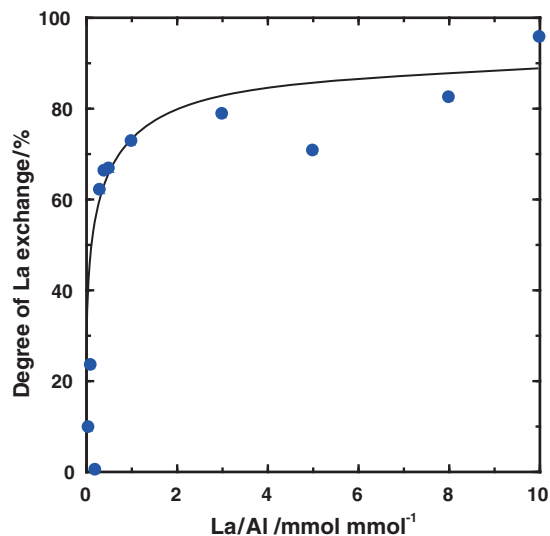
Figure 1. Effects of cation exchange on the lanthanum amounts against Al content of La,NaMOR.
