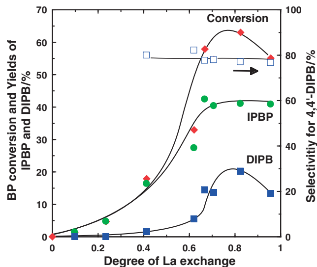
Figure 4. Effects of degree of La,NaMOR on the isopropylation of BP. Reaction conditions: BP, 100 mmol; catalyst, 0.5 g; propene, 0.8 MPa; temperature, 300 °C; period, 4 h.
