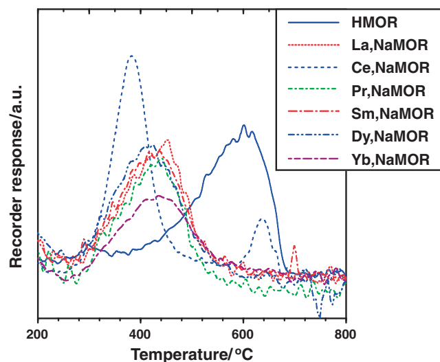
Figure 9. TG profiles of Ln,NaMORs used for the isopropylation of BP. Reaction conditions: BP, 100 mmol; temperature, 250 °C; propene pressure, 0.8 MPa; period, 4 h. TG measurement: sample, 10 mg; temperature programmed rate, 10 °C min -1 in an air stream.
